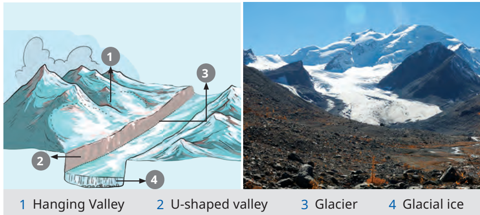
Fig. 2.18. U-shaped valley
